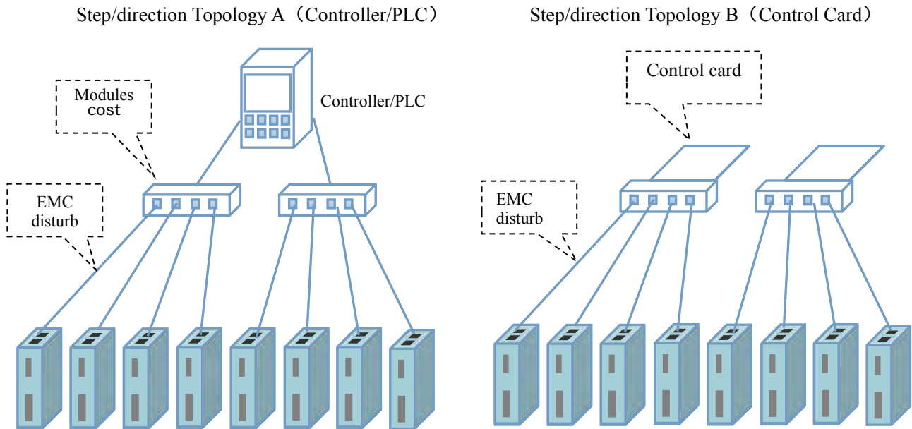
Figure 1.1: Step/direction Topology
