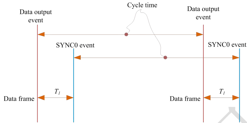
Figure 4.3: High performance synchronous mode
