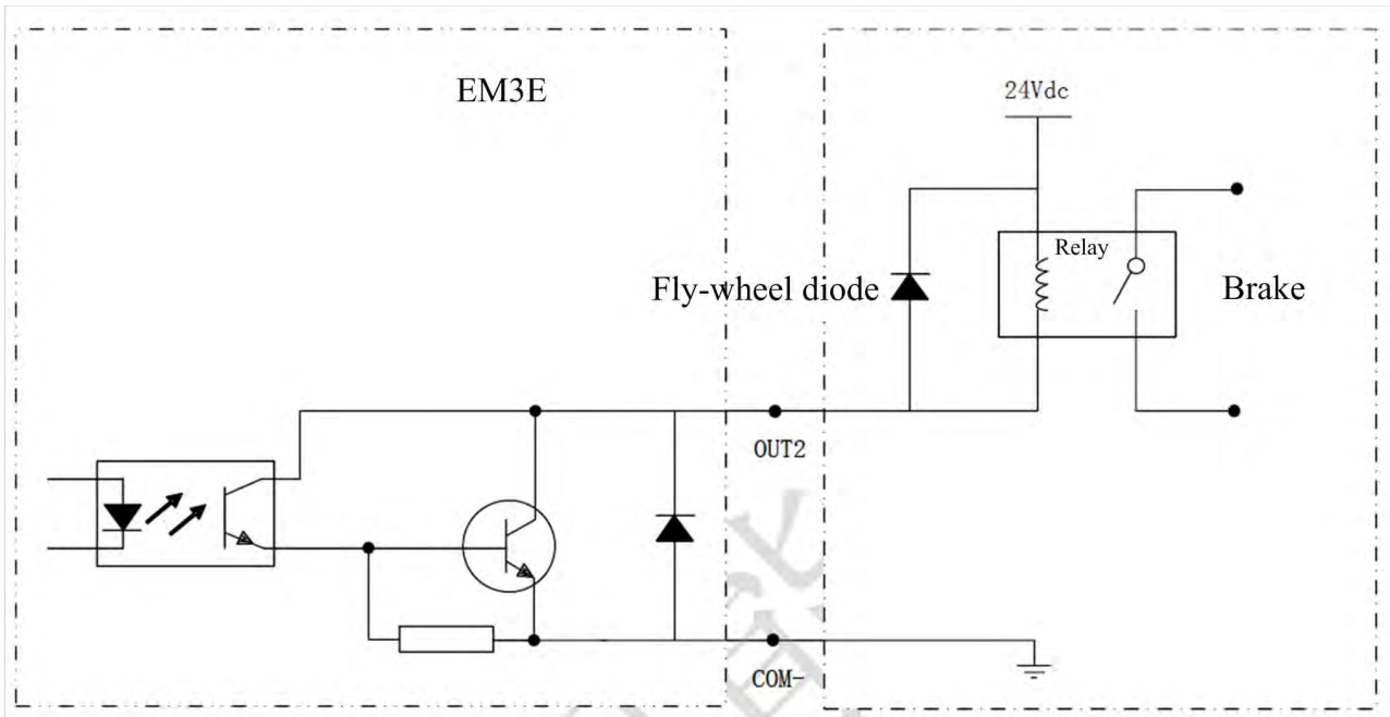
Figure 3.5 Brake Output Wiring
