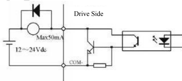
Figure 3.4 Output Interface Wiring
