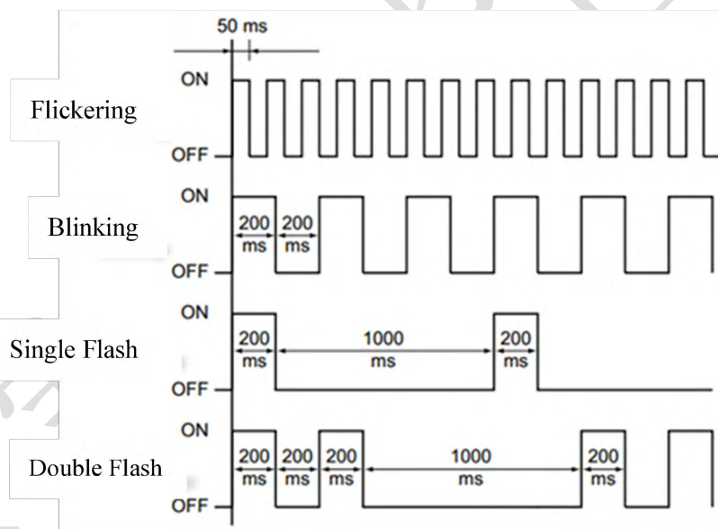
Figure 4.17: LED indicator lamp state
