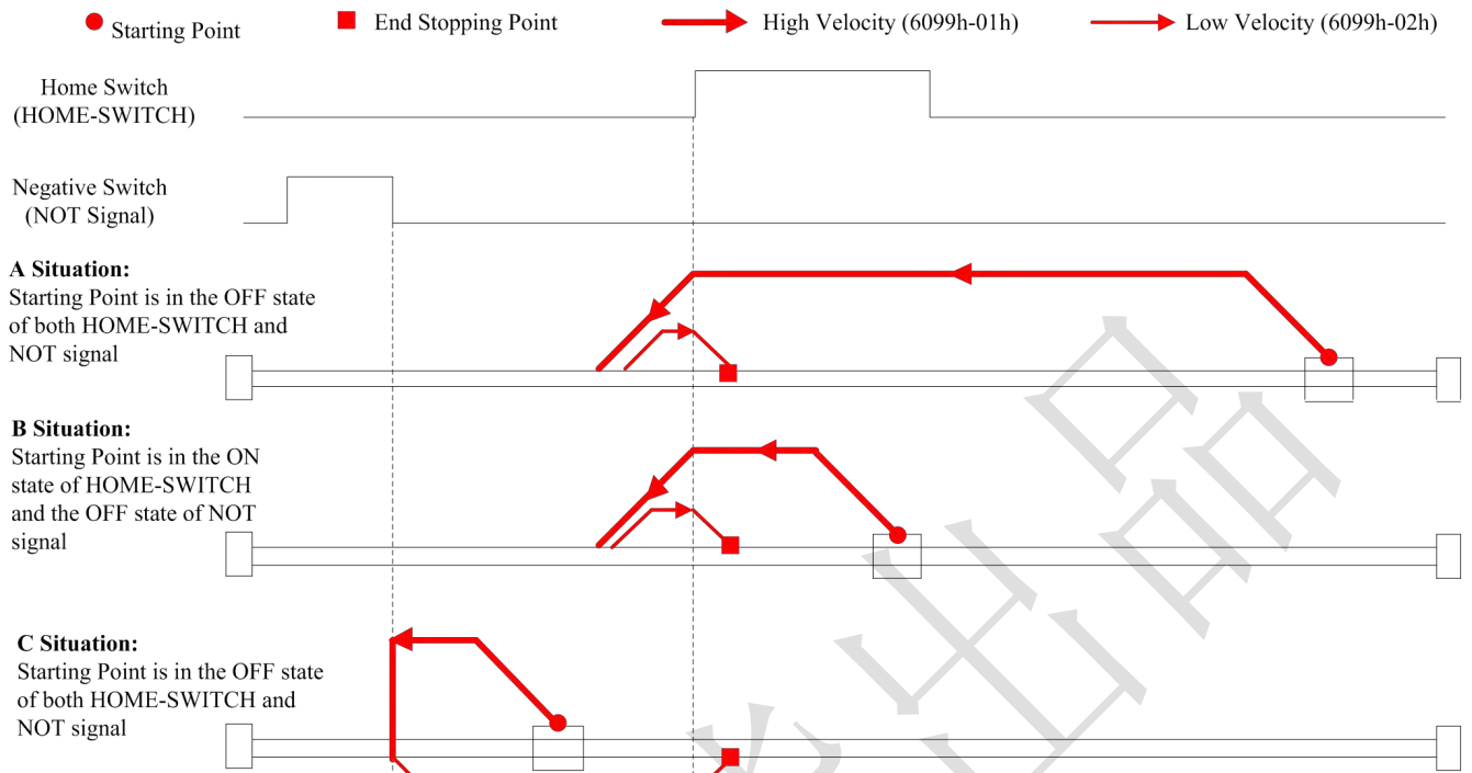
Figure 8.13 No.29 homing method
