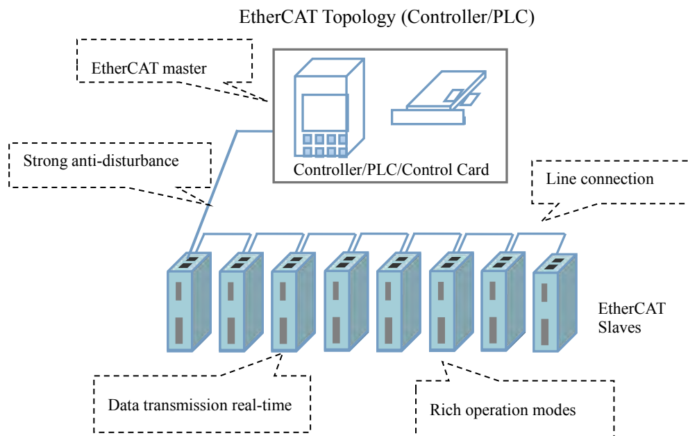
Figure 1.2: EtherCAT Topology
