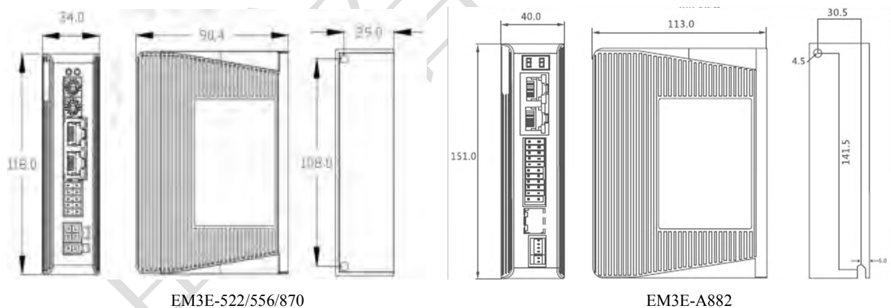
Figure 2.1 EM3E series mechanical drawing
